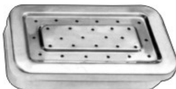
BOX WITH FILTER Size 15-310 100 x 50 mm 15-311 165 x 65 mm 15-312 250 x 100 mm 15-313 250 x 150 mm 15-314 250 x 200 mm 15-315 150 x 65 mm 15-316 170 x 70 mm 15-317 200 x 100 mm 15-318 250 x 125 mm 15-319 300 x 150 mm 15-320 300 x 200 mm 15-321 300 x 130 mm 15-322 320 x 150 mm 15-323 420 x 180 mm 15-324 460 x 125 mm 15-325 355 x 180 mm 15-326 300 x 180 mm 15-327 400 x 200 mm 15-328 510 x 200 mm
