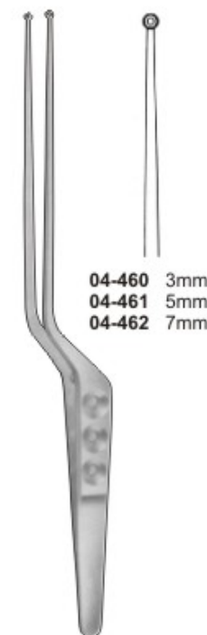
YASARGIL-SAMI Jaws Spoon-Shaped 24 cm, 9 1/4"
