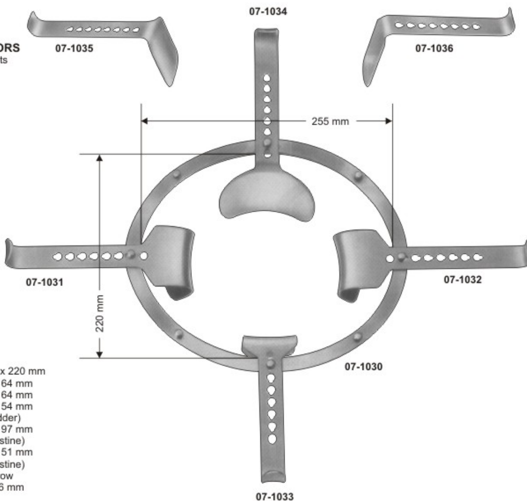
ABDOMINAL RETRACTORS for new-born and children
